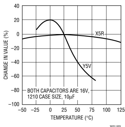
Figure 3. Ceramic Capacitor Temperature Characteristics
