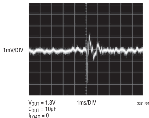
Figure 4. Noise Resulting from Tapping on a Ceramic Capacitor
