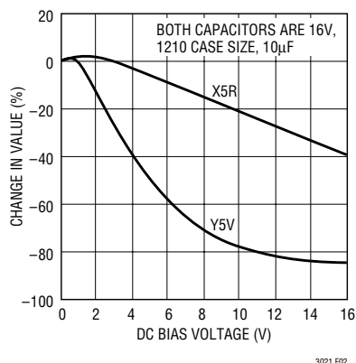
Figure 2. Ceramic Capacitor DC Bias Characteristics
