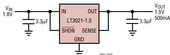
1.8V to 1.5V, 500mA VLDO Regulator
