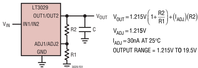
Figure 1. Adjustable Operation
