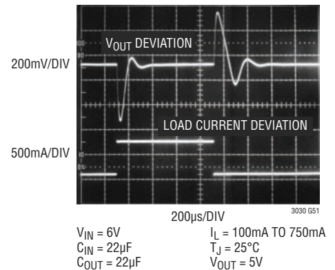
OUT1 Transient Response C_{BYP} = 0\text{pF}
