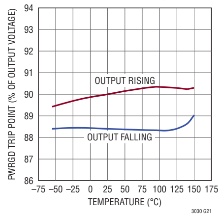
PWRGD1 or PWRGD2 Trip Point
