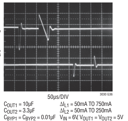
Channel-to-Channel Isolation
