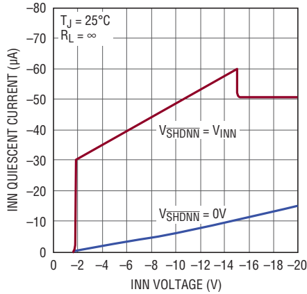
LT3032-15 INN Quiescent Current
