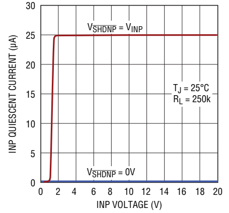
LT3032 INP Quiescent Current
