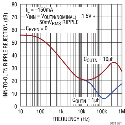
INN-to-OUTN Ripple Rejection
