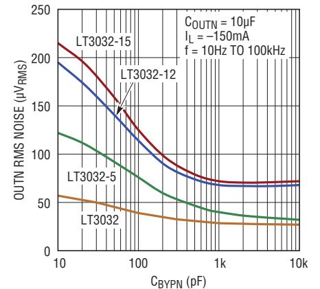
OUTN RMS Noise vs Bypass Capacitor
