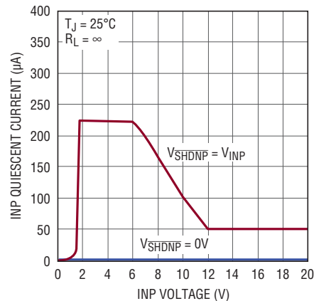
LT3032-12 INP Quiescent Current
