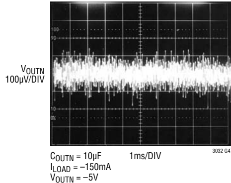
OUTN, 10Hz to 100kHz Output Noise, C_{BYPN} = 0.01\mu F
