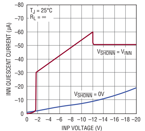
LT3032-12 INN Quiescent Current
