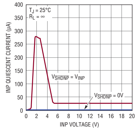
LT3032-5 INP Quiescent Current
