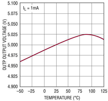
LT3032-5 OUTP Output Voltage
