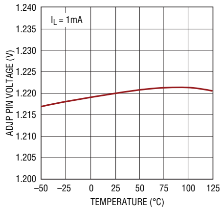
LT3032 ADJP Pin Voltage
