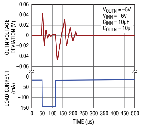
OUTN Transient Response C_{BYPN} = 0.01\mu F
