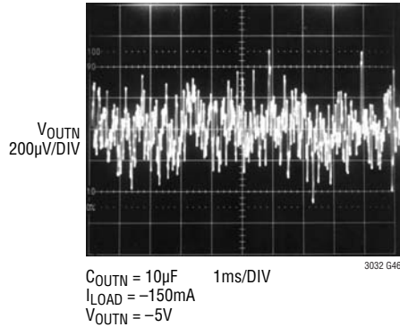
OUTN, 10Hz to 100kHz Output Noise, C_{BYPN} = 0
