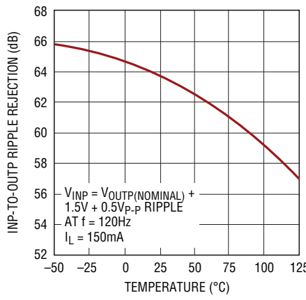
INP-to-OUTP Ripple Rejection
