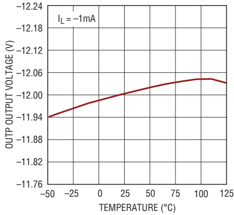
LT3032-12 OUTN Output Voltage
