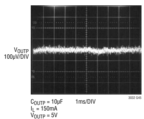
OUTP 10Hz to 100kHz Output Noise C_{BYP} = 0.01\mu F
