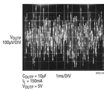
OUTP 10Hz to 100kHz Output Noise C_{BYP} = 0
