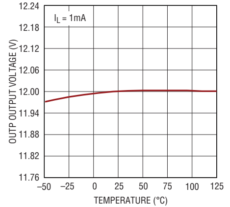
LT3032-12 OUTP Output Voltage
