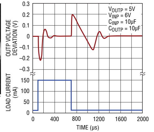
OUTP Transient Response C_{BYPN} = 0
