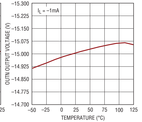
LT3032-15 OUTN Output Voltage
