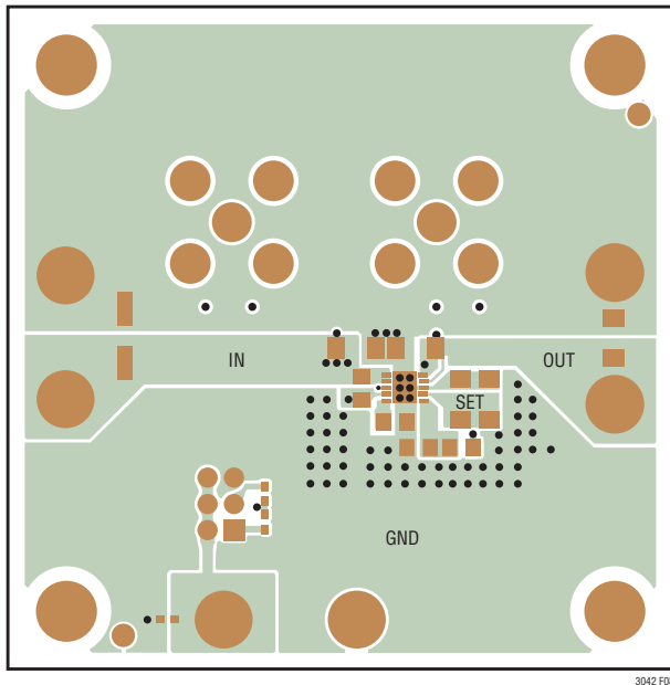
Figure 8. Example DFN Layout
