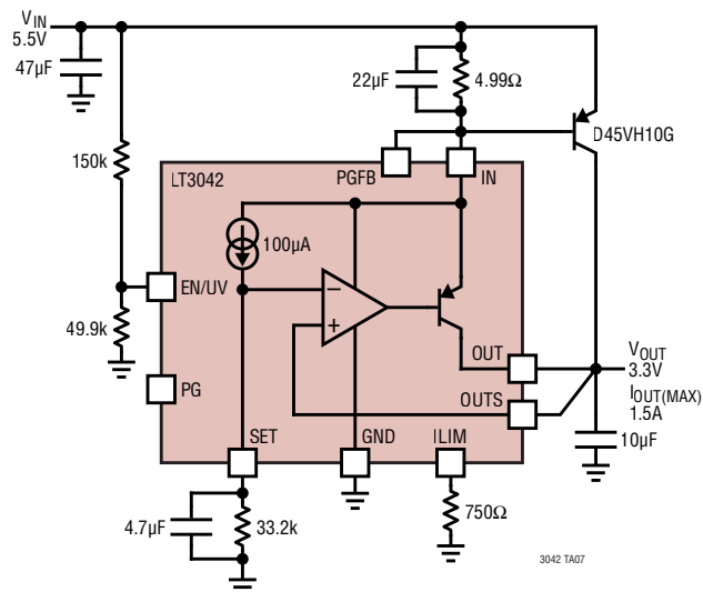
Ultralow Noise Higher Current Regulator with External PNP
