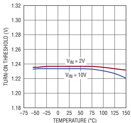
EN/UV Turn-On Threshold
