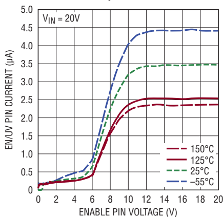
Enable Pin Input Current
