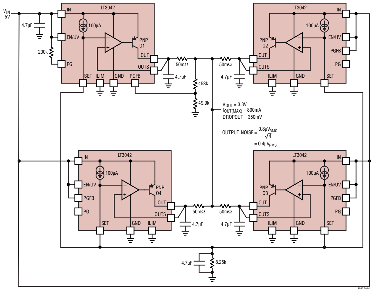
Paralleling Multiple LT3042s for Higher Output Current
