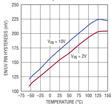
EN/UV Pin Hysteresis
