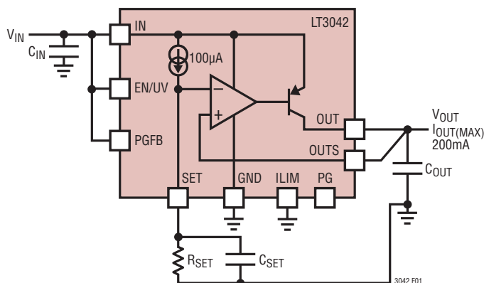
Figure 3. C_{OUT} and C_{SET} Connections for Stability
