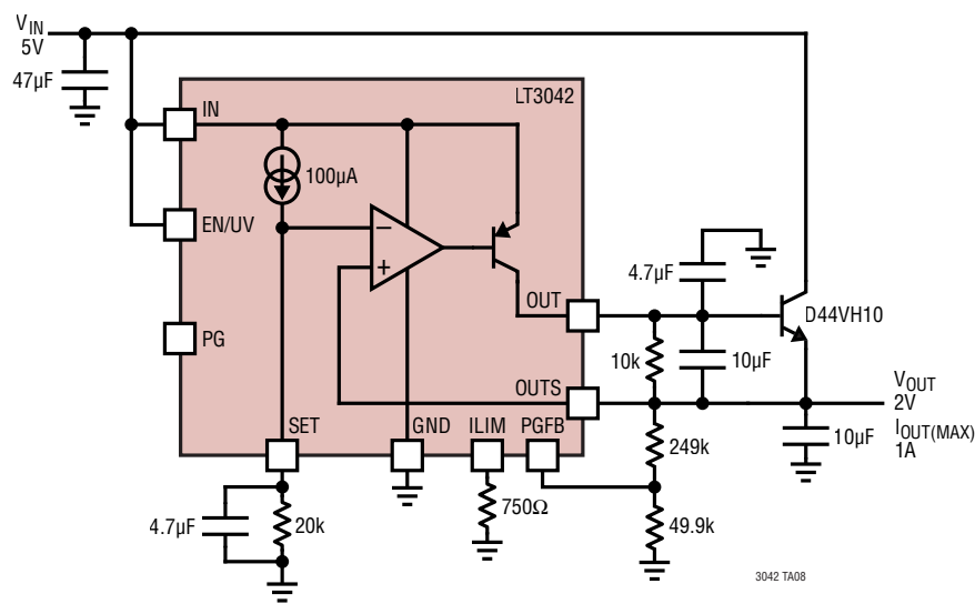
Ultralow Noise Higher Current Regulator with External NPN
