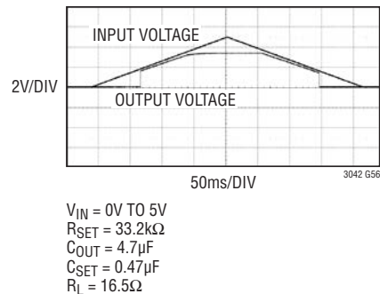
Input Supply Ramp-Up and Ramp-Down
