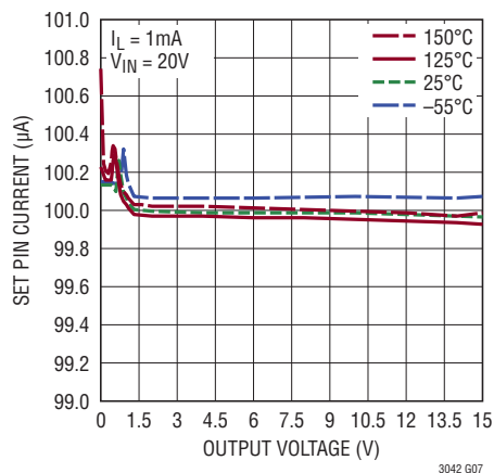
SET Pin Current
