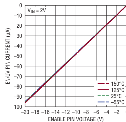
Enable Pin Current
