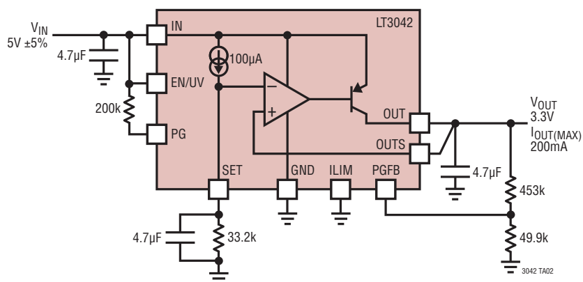
5V V_{IN} to 3V V_{OUT} with 0.8 \mu V RMS Integrated Noise
