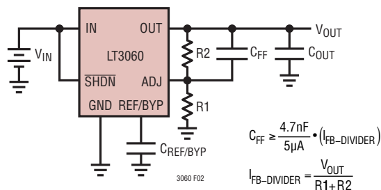
Figure 2. Feedforward Capacitor for Fast Transient Response
