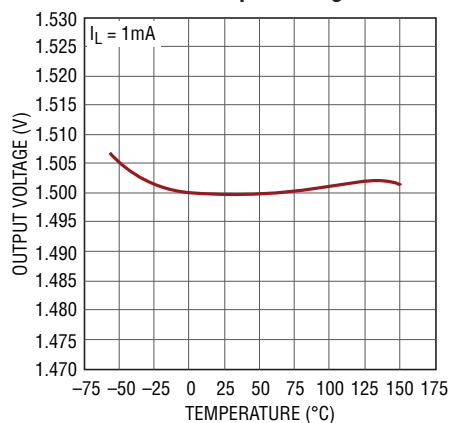
LT3060-1.5 Output Voltage
