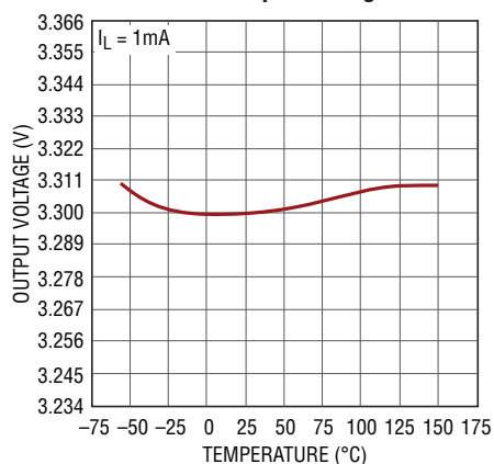
LT3060-3.3 Output Voltage
