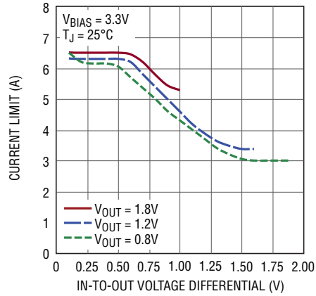
Current Limit vs V_{IN} - V_{OUT}
