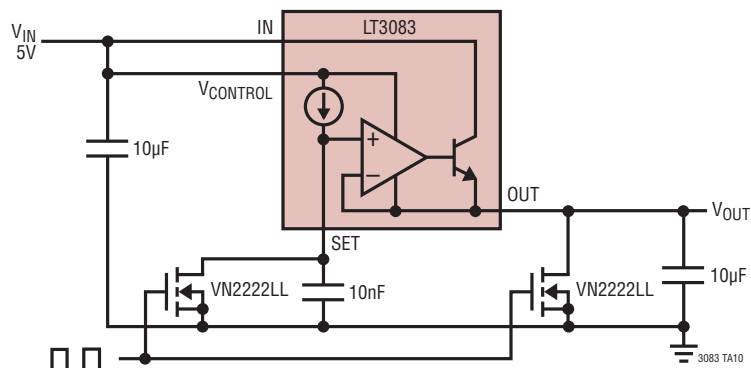
Ramp Generator
