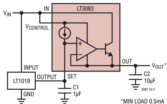
Reference Buffer
