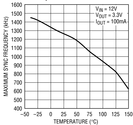
Maximum Sync Frequency vs Temperature
