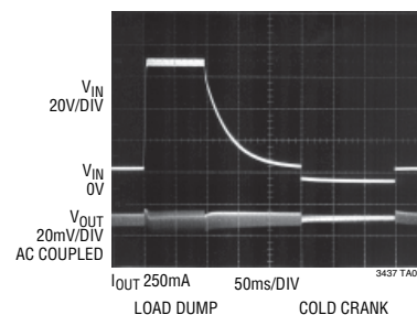
Input Voltage Transient Response
