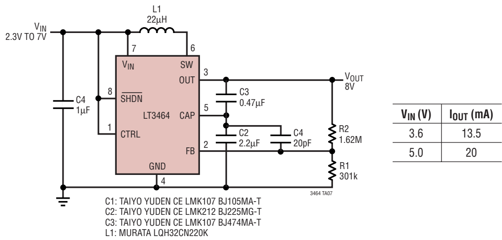
8V Output Converter with Output Disconnect
