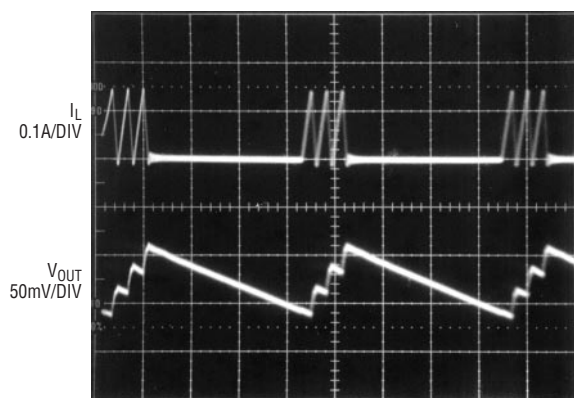
Operating Waveforms
