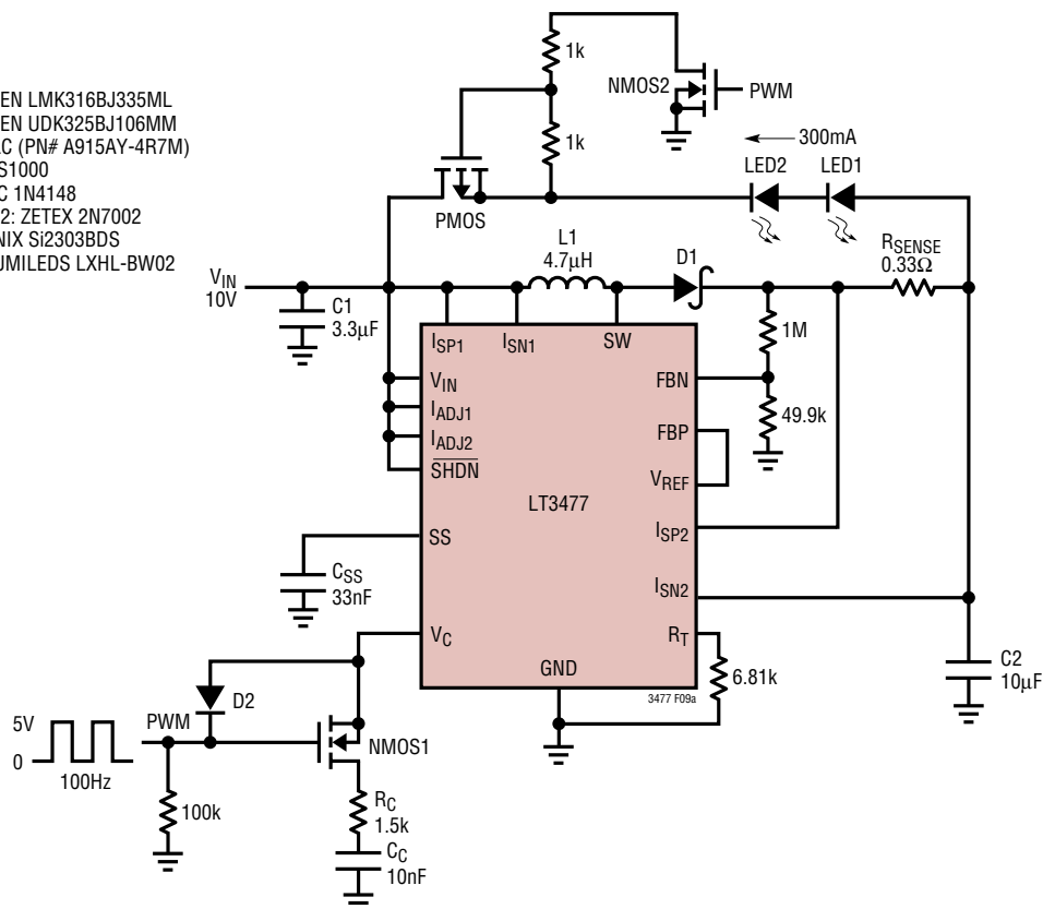
Figure 9a. 10V to 2 White LEDs: Buck-Boost Mode with PWM Dimming
