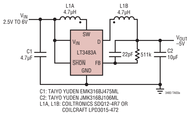
-5V Step-Up/Step-Down Converter
