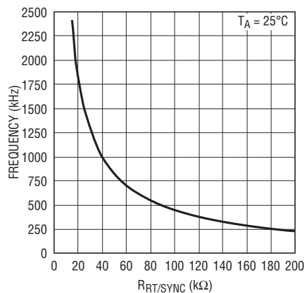
Frequency vs R_{RT}/\text{SYNC}
