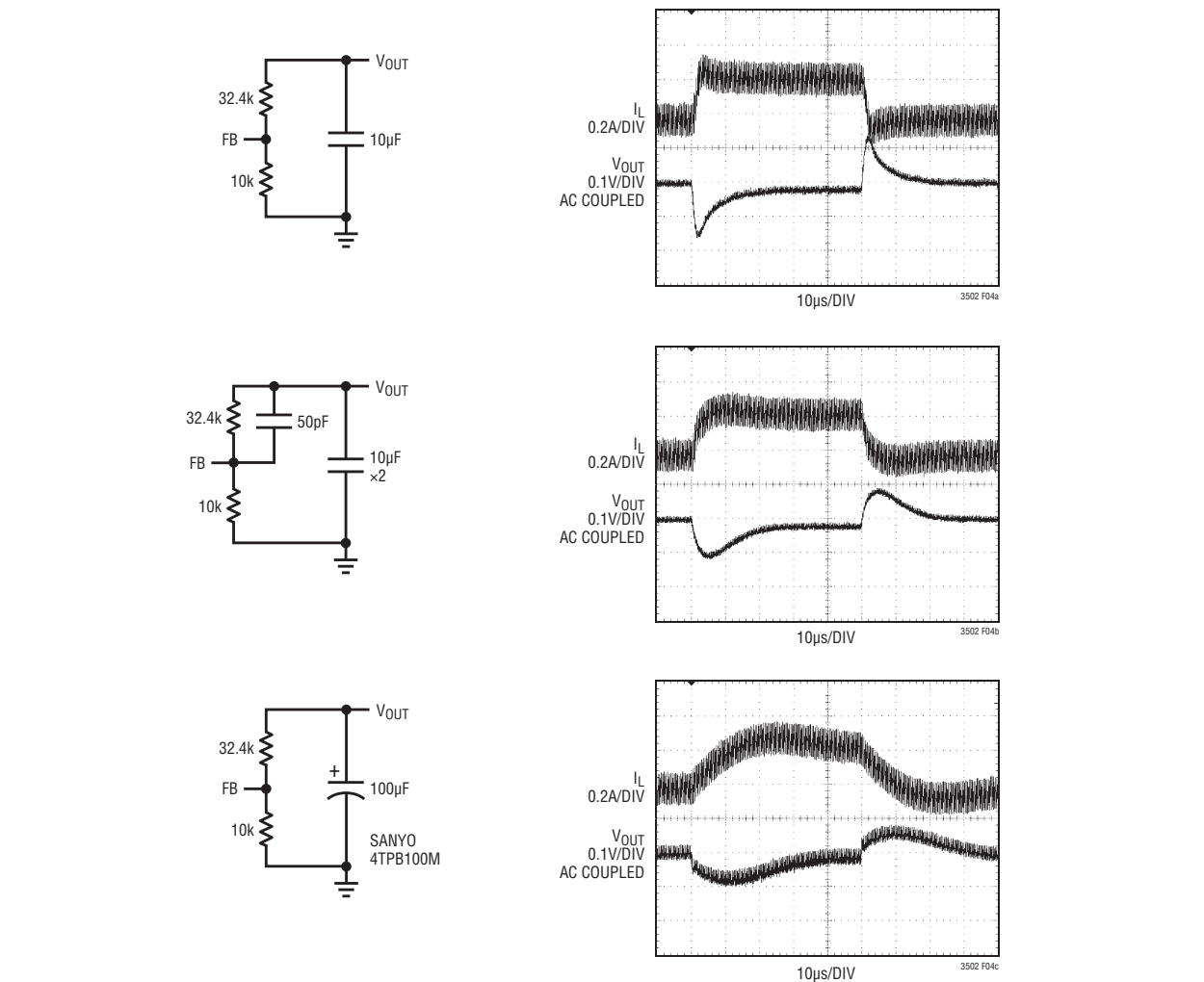
Figure 4. Transient Load Response of the LT3502A with Different Output Capacitors as the Load Current is Stepped from 150mA to 400mA. V_{IN} = 12V , V_{OUT} = 3.3V , L = 6.8\mu H
