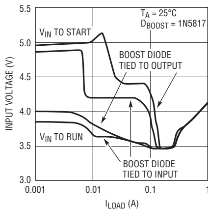
Minimum Input Voltage, V_{\text{OUT}} = 3.3\text{V} (LT3506A)
