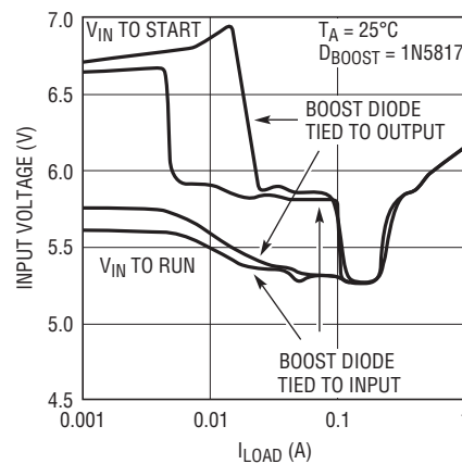
Minimum Input Voltage, V_{\text{OUT}} = 5\text{V} (LT3506A)
