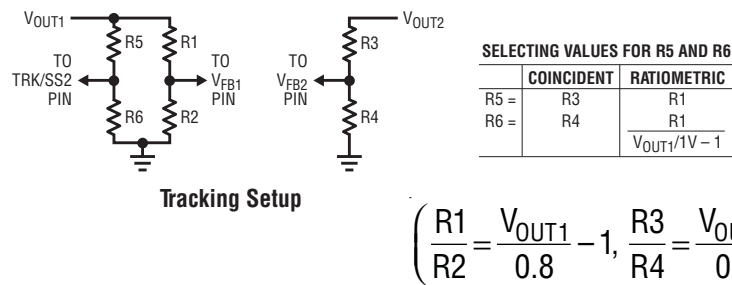
Figure 9. Setup for Coincident and Ratiometric Tracking
