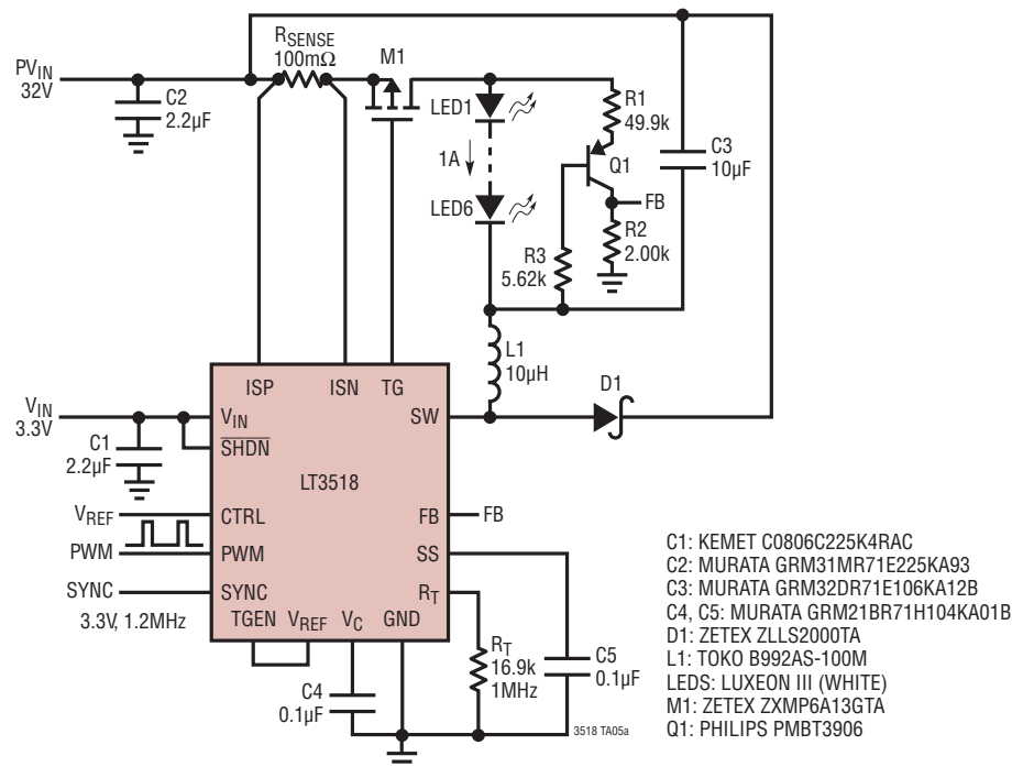
Buck Mode 1A LED Driver with Open LED Protection and Sync Input
