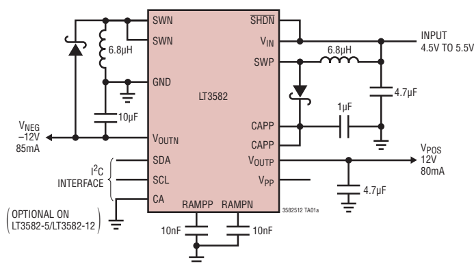
±12V Supplies from a Single 5V Input
