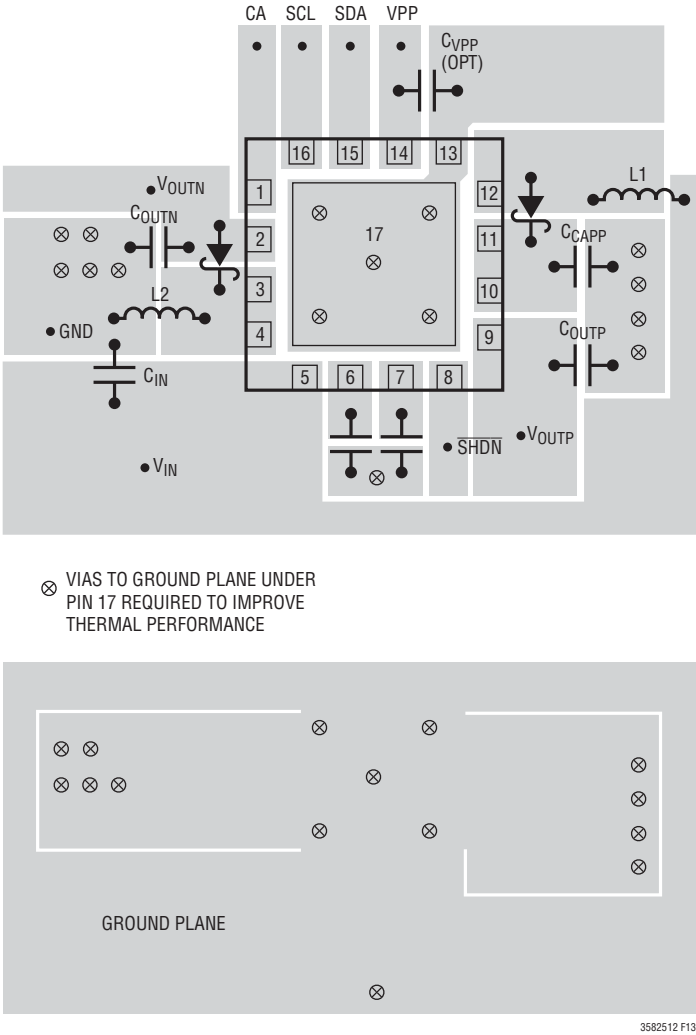
Figure 12. Suggested Component Placement (Not to Scale)
