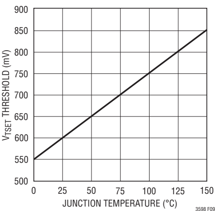
Figure 9. TSET Pin Threshold
