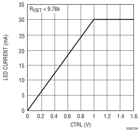
Figure 4. LED Current vs CTRL Voltage
