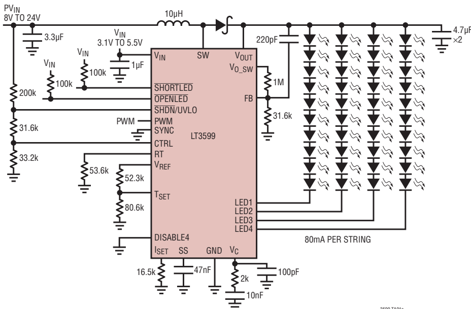
90% Efficient 12W LED Driver
