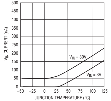
V_{IN} Current (Shutdown)
