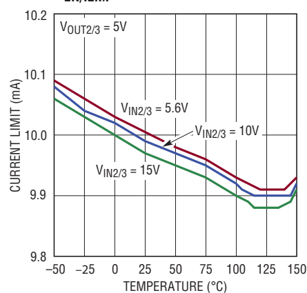
LD0s: External Current Limit, R_{EN/ILIM} = 31.6k
