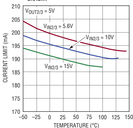
LD0s: External Current Limit, R_{EN/ILIM} = 1.54k
