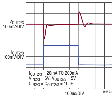
LD0s: Transient Response
