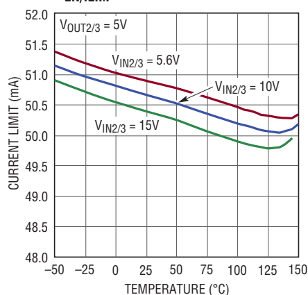
LD0s: External Current Limit, R_{EN/ILIM} = 6.19k
