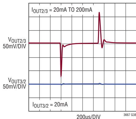
LD0s: Channel-to-Channel Isolation
