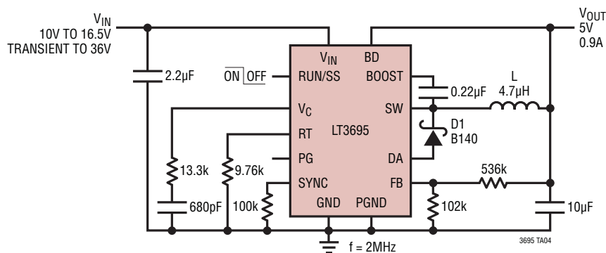
5V, 2MHz Step-Down Converter
