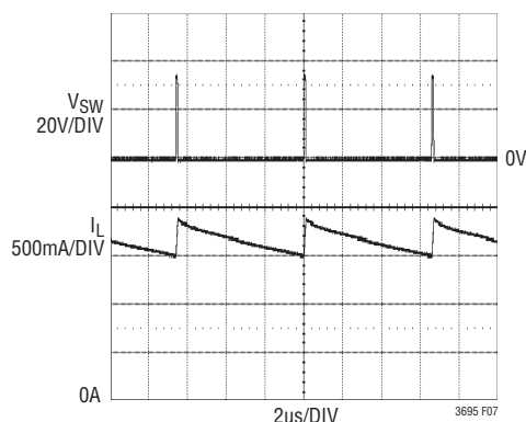
Figure 7. The LT3695 Reduces its Frequency to Protect Against Shorted Output with 36V Input
