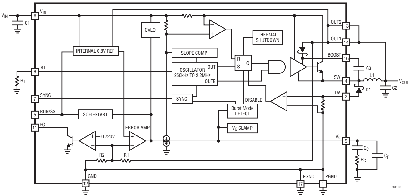
LT3695-3.3/LT3695-5
