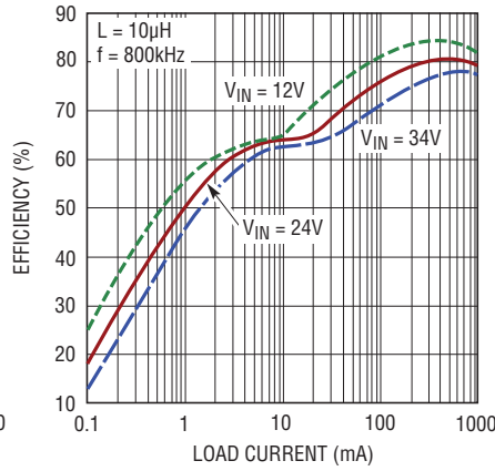
Efficiency ( V_{OUT} = 3.3V , SYNC = 0V)
