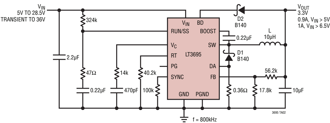
Fully Tolerant 3.3V Step-Down Converter with Soft-Start
