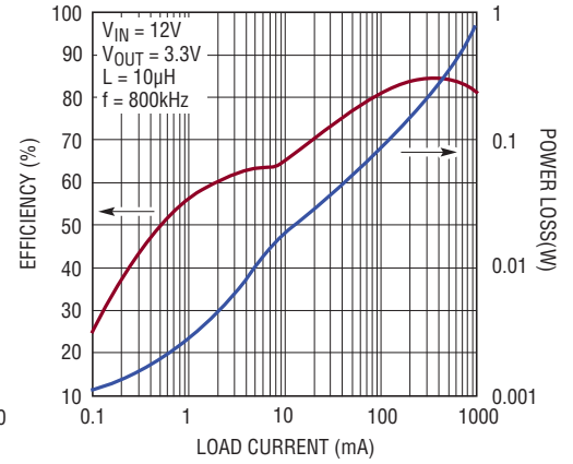
Efficiency ( V_{OUT} = 3.3V , SYNC = 0V)
