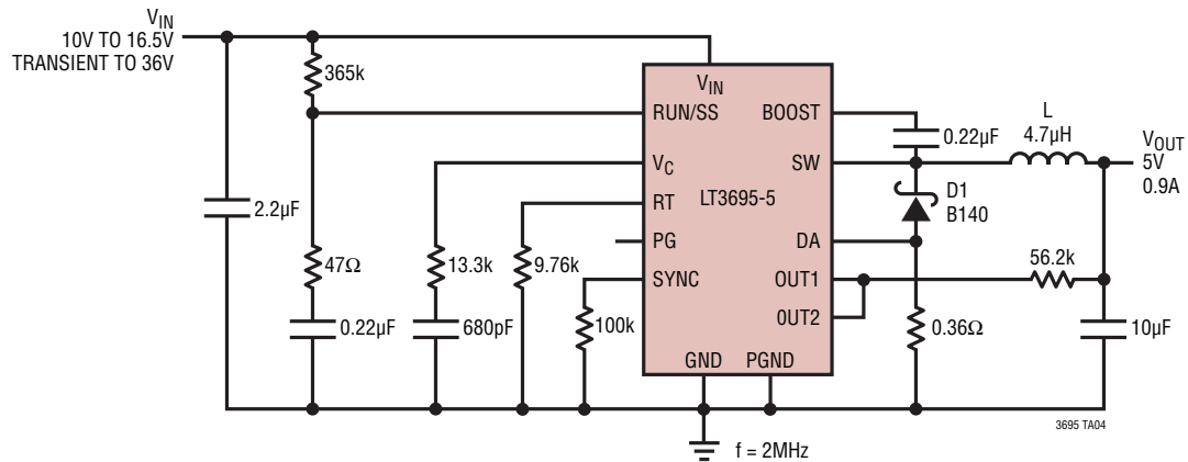
Fully Tolerant 5V Step-Down Converter with Soft-Start
