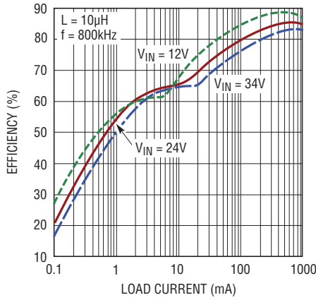
Efficiency ( V_{OUT} = 5V , SYNC = 0V)
