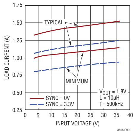
Maximum Load Current
