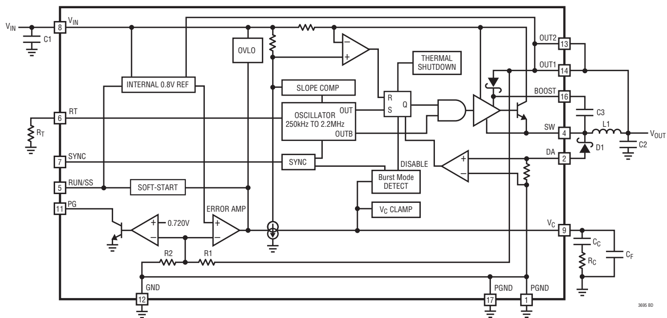
LT3695-3.3/LT3695-5
