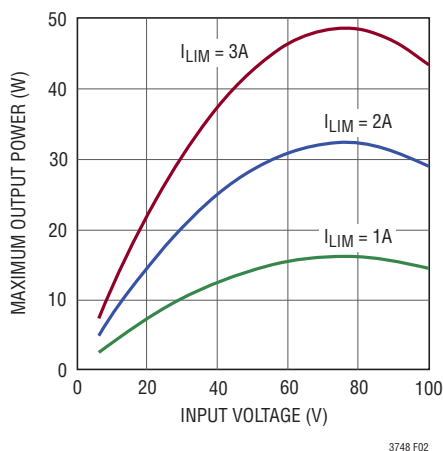
Figure 2. Maximum Output Power at 12V OUT with 150V V_{\text{DS(MAX)}} and I_{\text{LIM}} = 1\text{A}, 2\text{A}, 3\text{A}
