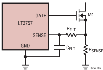
Figure 5. The RC Filter on SENSE Pin
