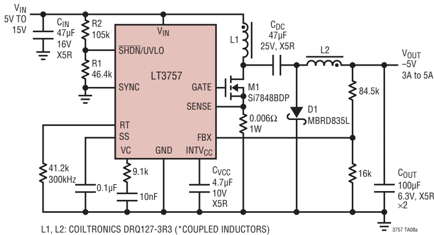
High Efficiency Inverting Power Supply
