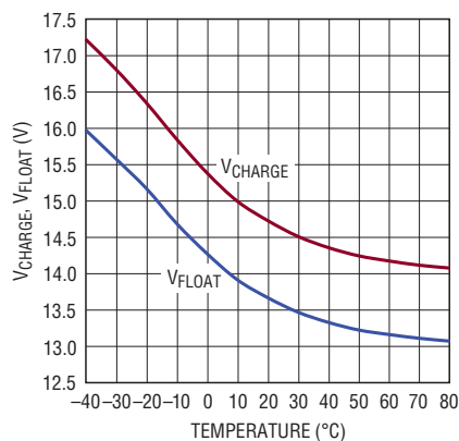
V CHARGE , V FL0AT vs Temperature
