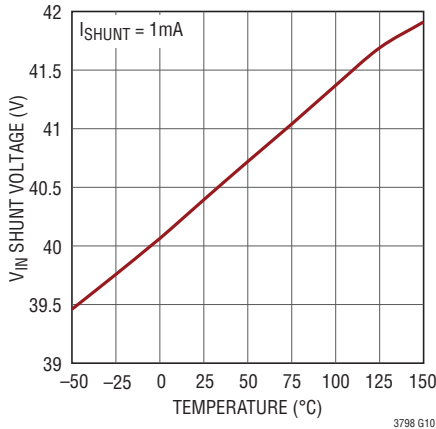
V_{IN} Shunt Voltage vs Temperature
