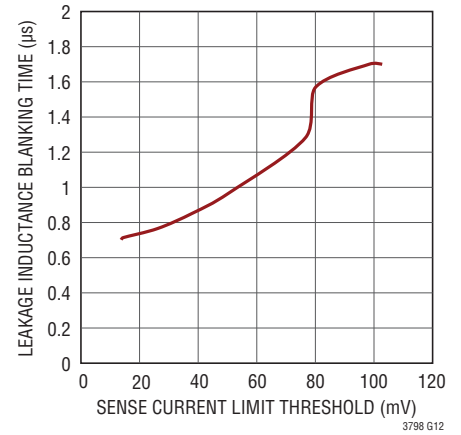
Leakage Inductance Blanking Time vs SENSE Current Limit Threshold
