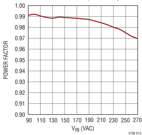
Power Factor vs Input Voltage
