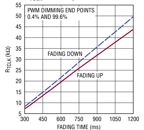
R_{TCLK} vs Fading Time
