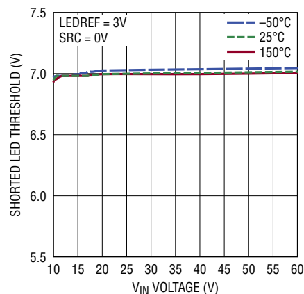
Shorted LED Threshold Falling vs V_{IN} , Temperature for V_{STH}[1:0] = 10
