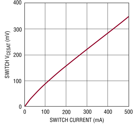
Switch V_{\text{CESAT}}
