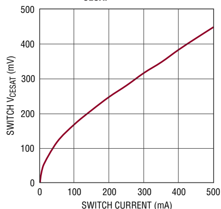
Switch V_{\text{CESAT}}
