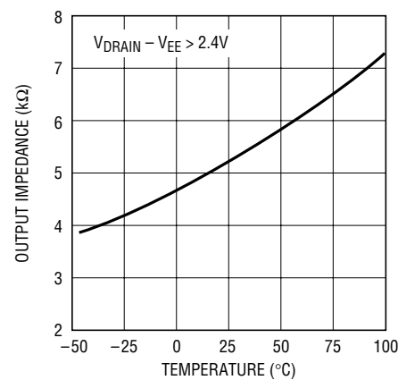
PWRGD Output Impedance vs Temperature (LT4250H)
