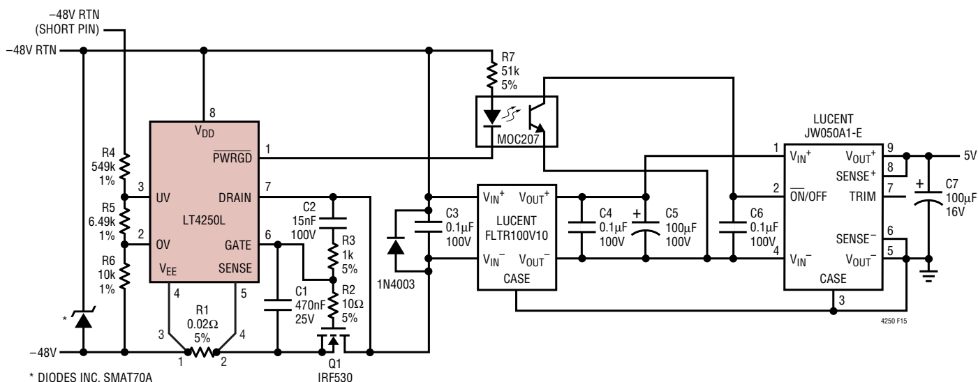
Figure 15. Typical Application Using a Filter Module
