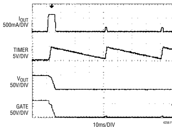
Figure 11. RETRY Waveforms
