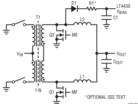
Figure 4d. Typical Synchronous Push-Pull Current-Doubler Converter with Bias Generator
