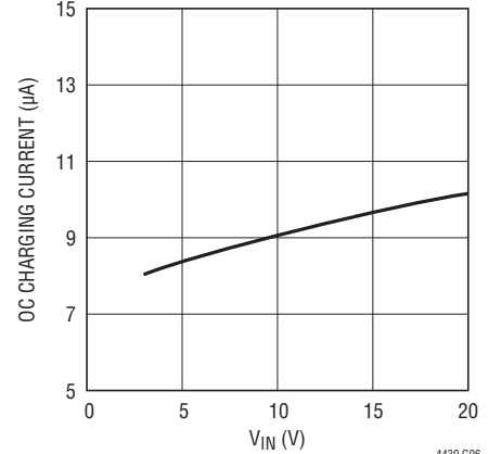
OC Charging Current vs Input Voltage
