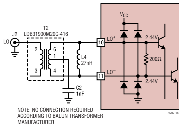
Figure 6. LO Input Equivalent Circuit with External Matching
