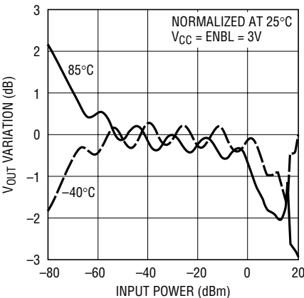
V OUT Variation vs Input Power at 100MHz
