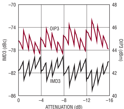
Two-Tone IMD3 and OIP3 vs Attenuation at 100MHz
