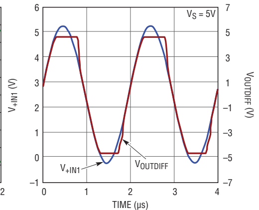
Overdrive Recovery
