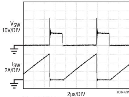
Switching Waveform
