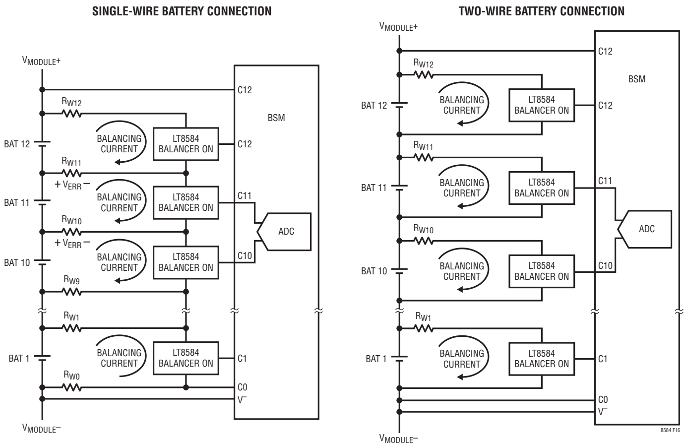
Figure 16. LT8584 Battery Connections
