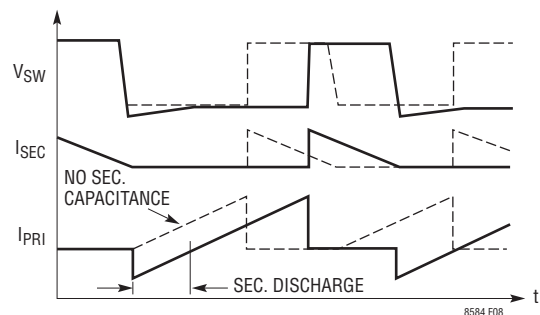
Figure 8. Effect of Secondary Winding Capacitance
