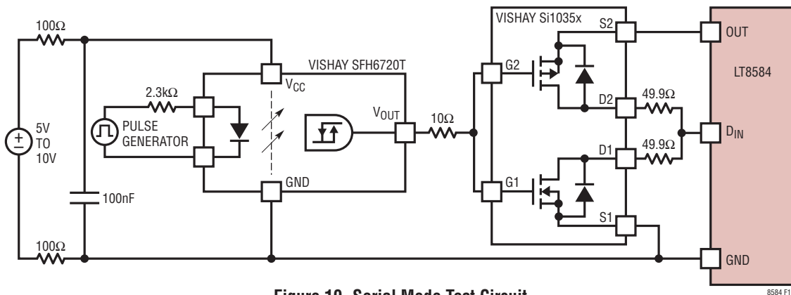
Figure 19. Serial Mode Test Circuit
