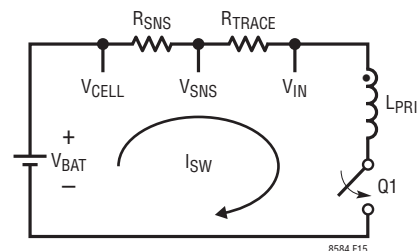
Figure 15. R_{TRACE} Minimization
