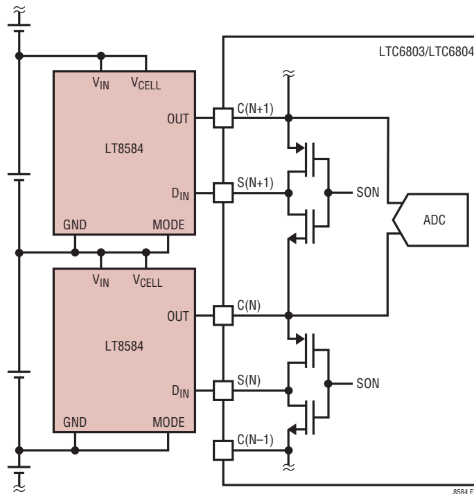
Figure 18. LTC6803/LTC6804 Simplified Connections
