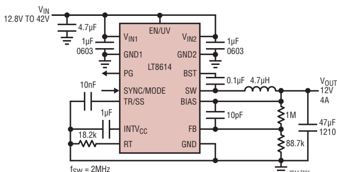
2MHz 12V, 4A Step-Down Converter
