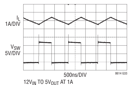
Switching Waveforms
