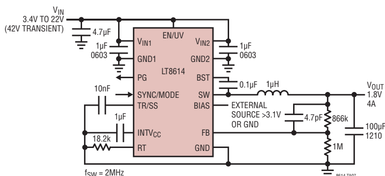
2MHz 1.8V, 4A Step-Down Converter
