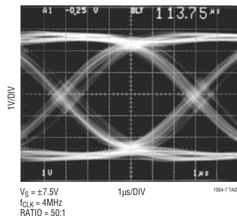
Eye Diagram
