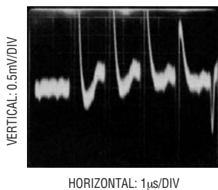
Figure 16. Poor Reference Settling Can Cause A/D Errors
