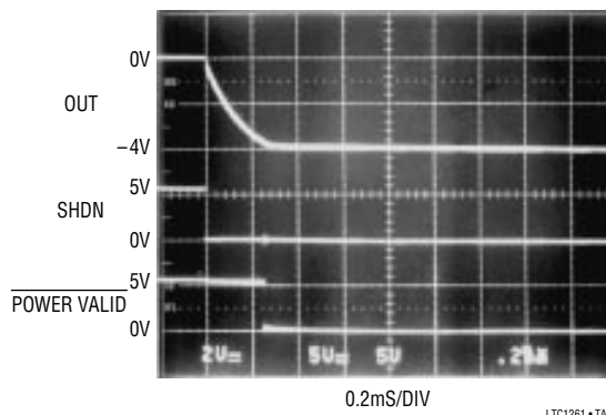
Waveforms for -4\text{V} Generator with Power Valid
