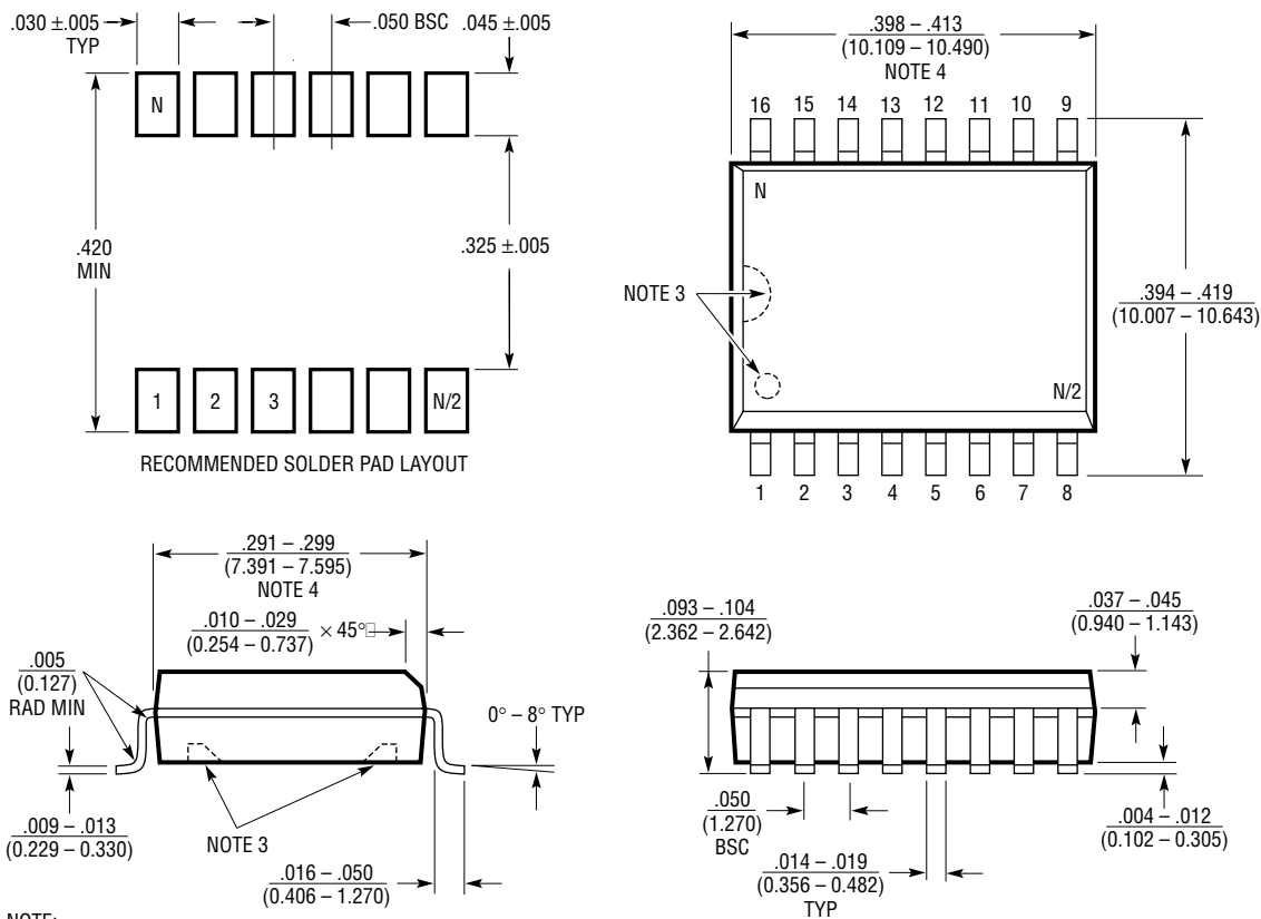
SW Package 16-Lead Plastic Small Outline (Wide .300 Inch) (Reference LTC DWG # 05-08-1620)
