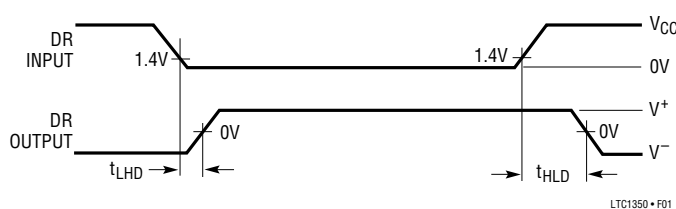
Figure 1. Driver Propagation Delay Timing
