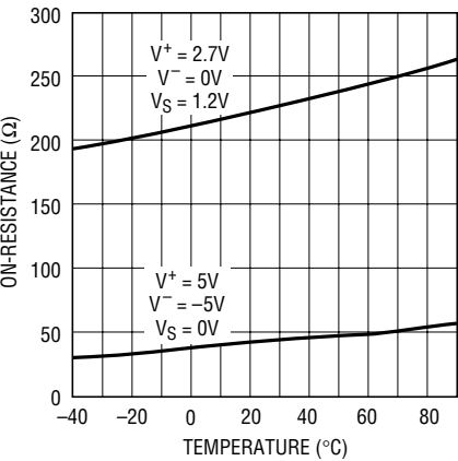
On-Resistance vs Temperature
