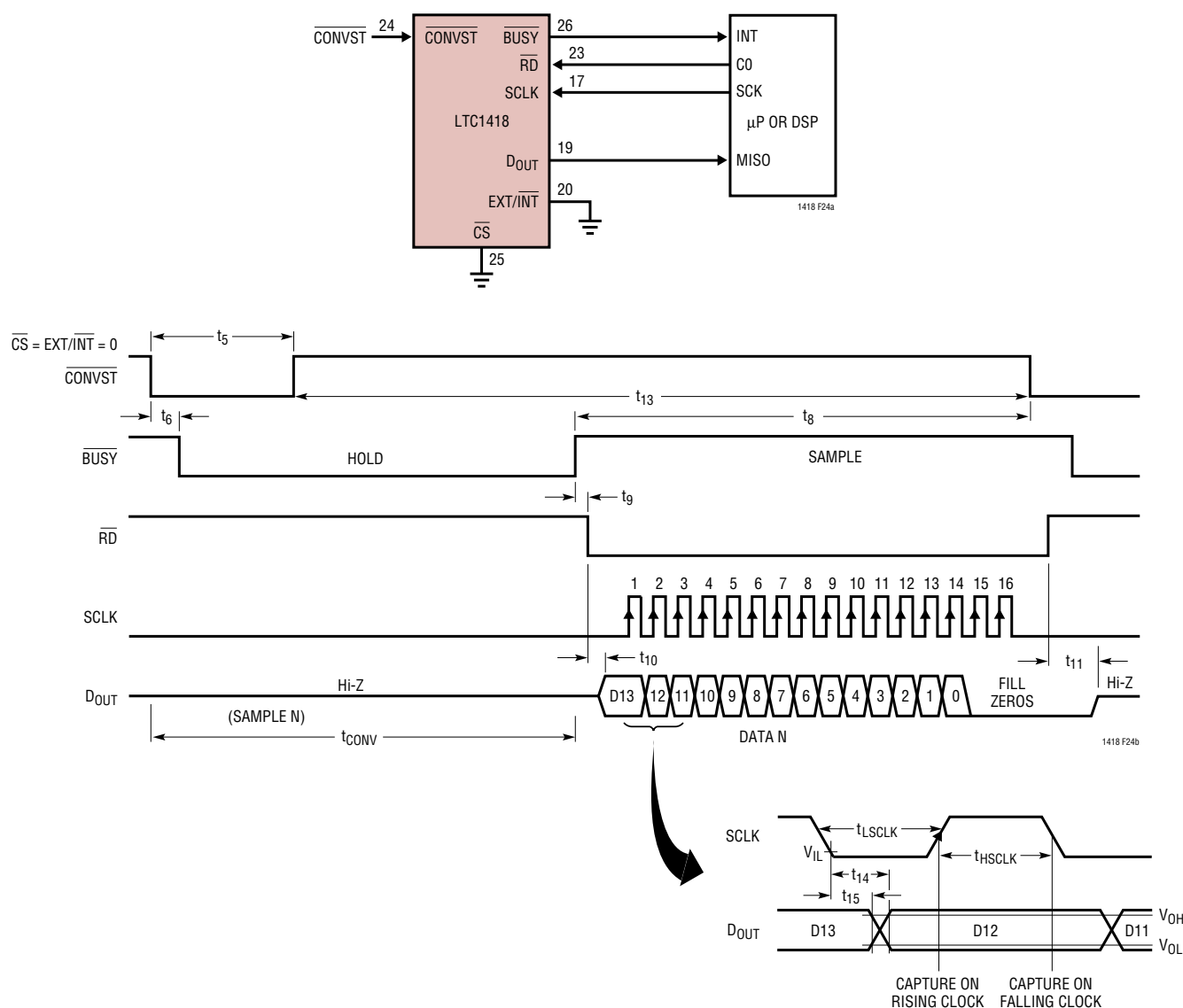
Figure 24. Internal Conversion Clock Selected. Data Transferred After Conversion Using an External SCLK. BUSY\uparrow Indicates End of Conversion
