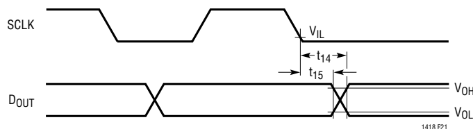
Figure 21. SCLK to \text{D}_{\text{OUT}} Delay
