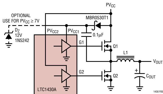
Figure 5. Doubling Charge Pump
